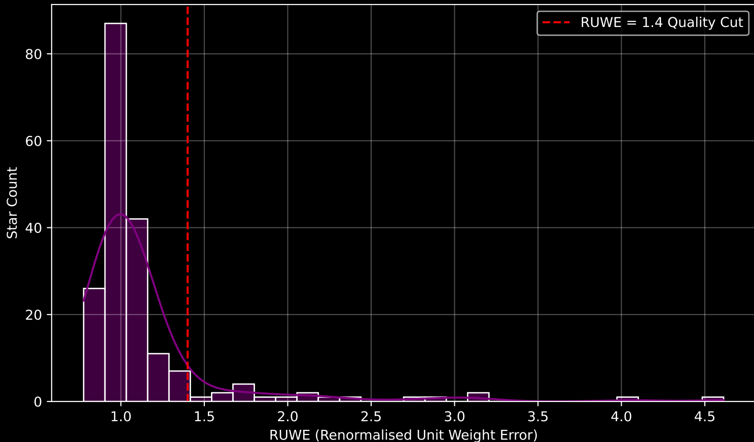
GAPOGEE DR17 Field [195+32_MGA] RUWE Distribution (n= 192)
