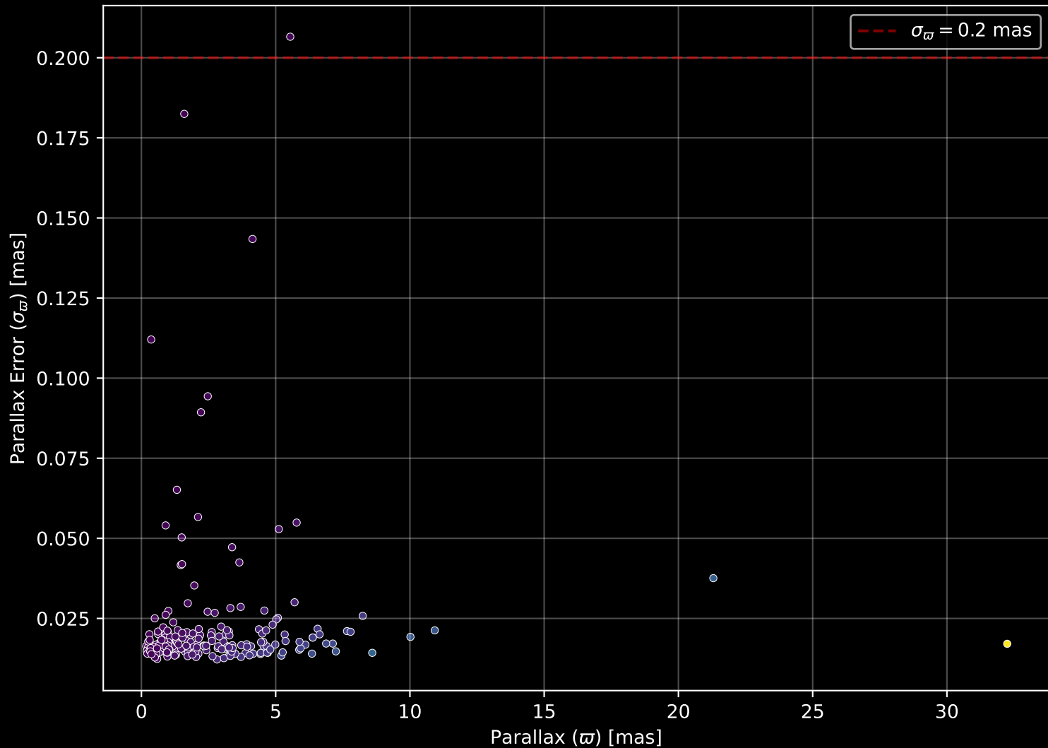
APOGEE DR17 Field: [195+32_MGA] Parallax Quality (n= 197)
