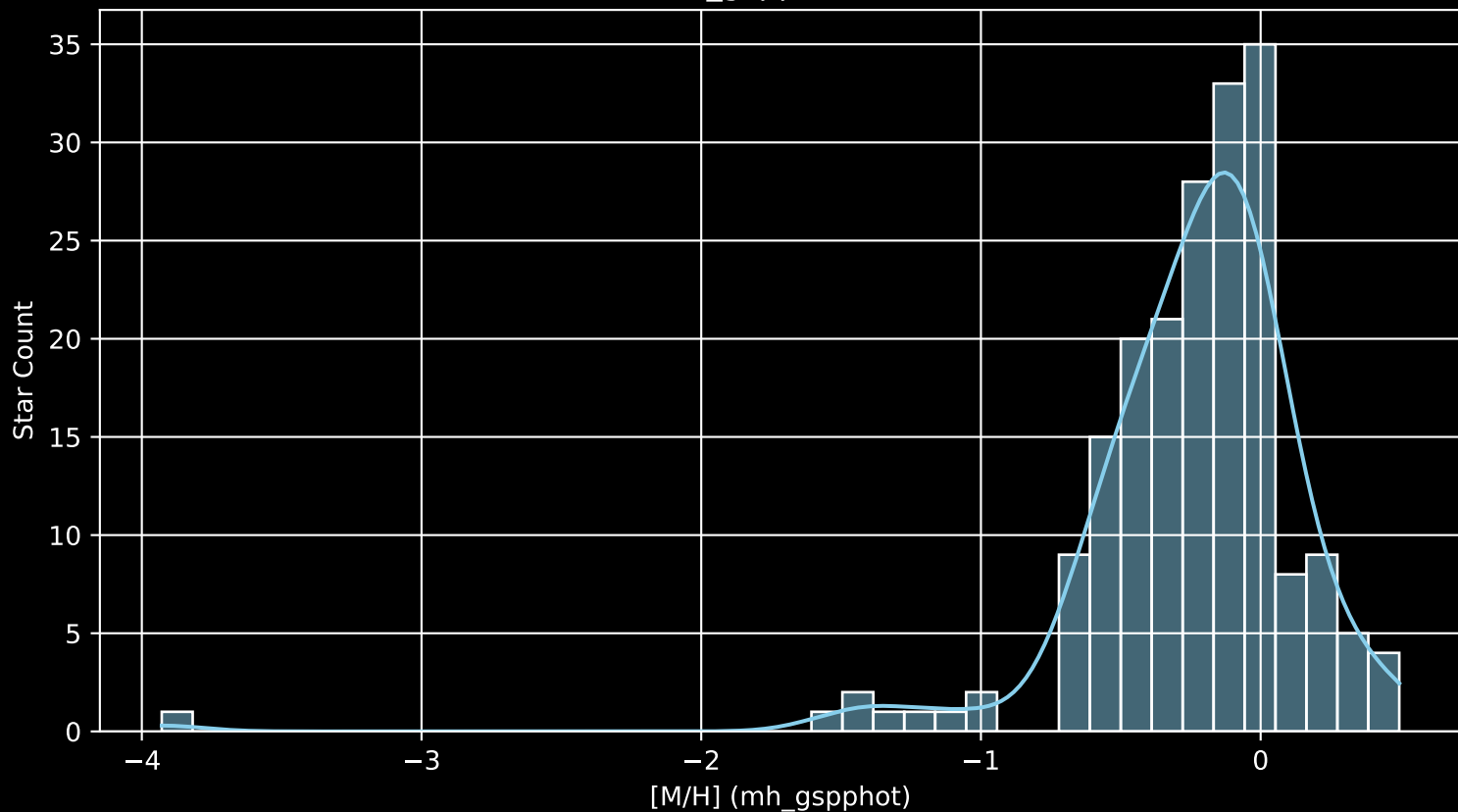
APOGEE DR17 Field: [195+32_MGA [M/H] (mh_gspphot) (n= 196)
