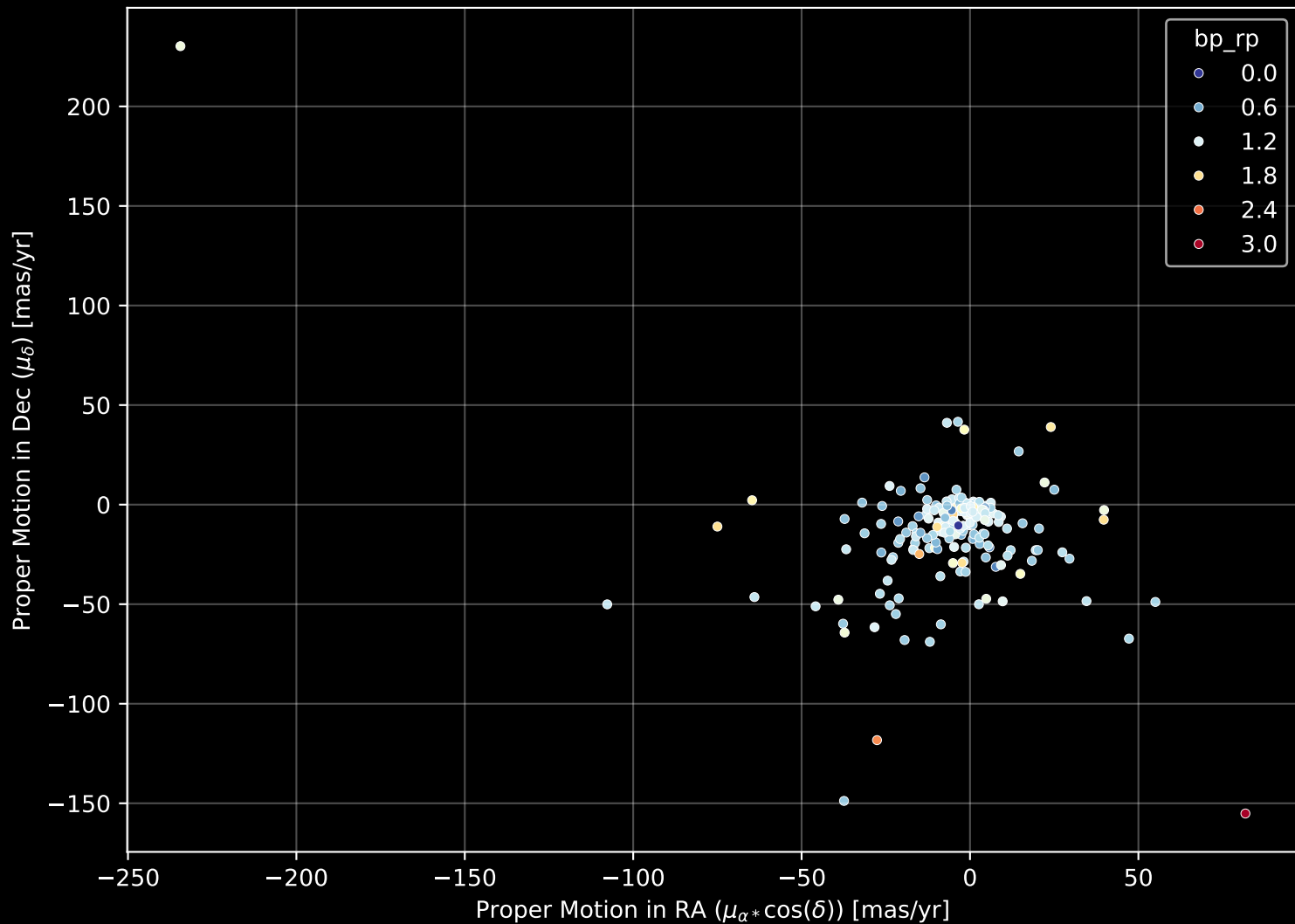
APOGEE DR17 Field: [195+32_MGA] Proper Motion Diagram (n= 197)
