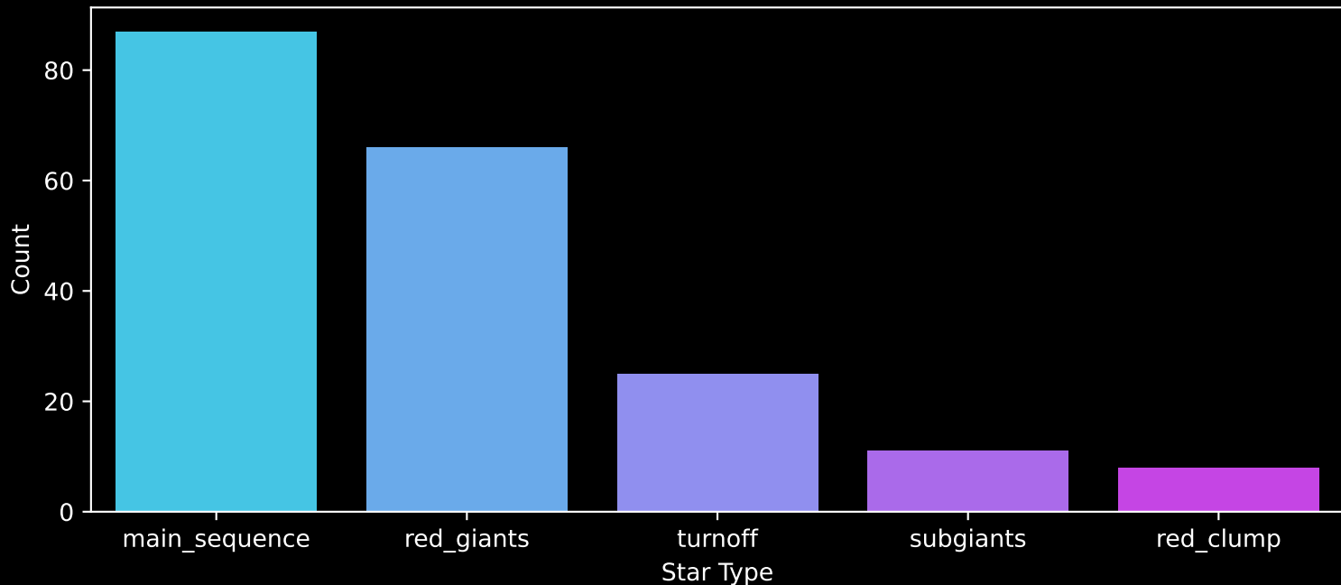
APOGEE DR17 Field: [195+32_MGA] Count plot of Star Type
