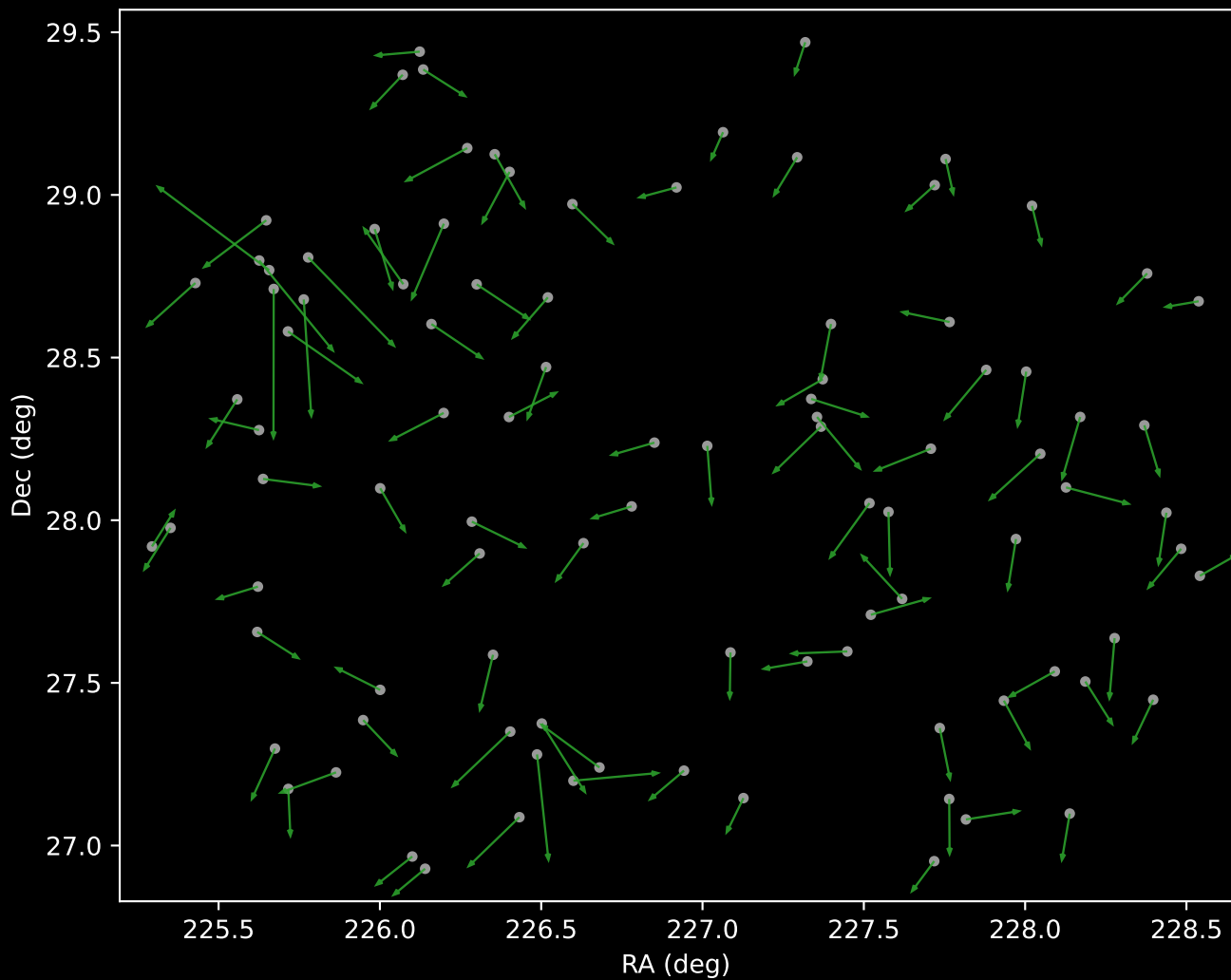
APOGEE DR17 Cluster 4 Proper Motion Vectors (n=97)
